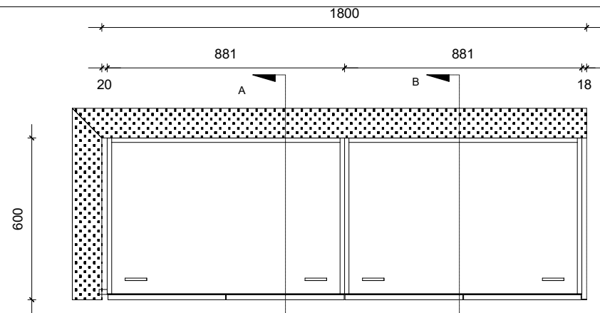
BUILT-IN ROBE Plan Scale: 1 : 20
