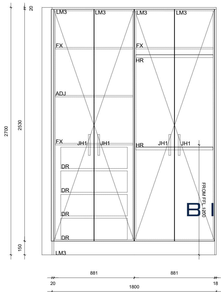
BUILT-IN ROBE Elevation A Scale: 1 : 20
